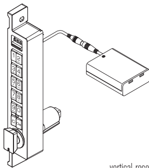
vertical recess mount with wired battery pack
