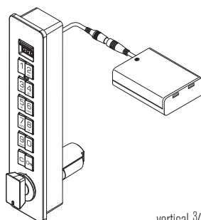
vertical 3/4 inch recess mount with integrated battery pack
